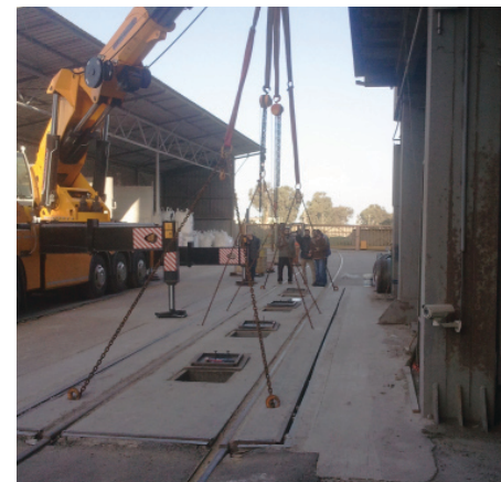
Train cars weighing bridge installation
