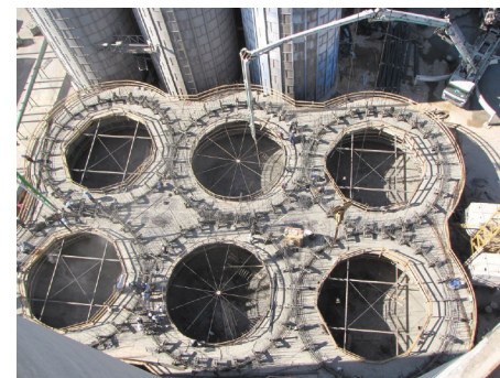
Concrete silo 20,000 metric ton- walls casting
